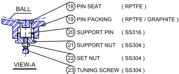
SUPPORT BALL DESIGN( 6" , 8" , 10",12" )
