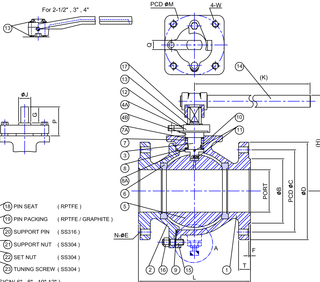
SUPPORT BALL DESIGN( 6" , 8" , 10",12" )
